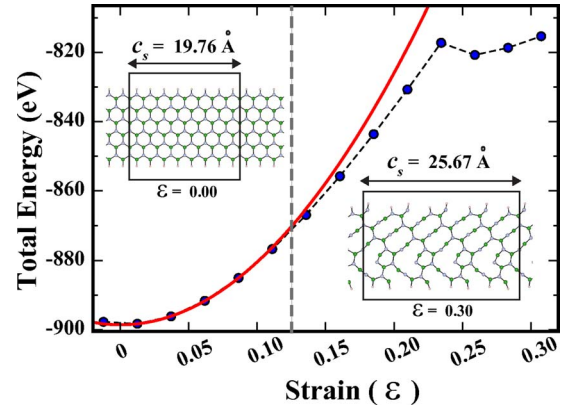
FIG. 9. (Color online) Variation in the total energy of hydrogen-saturated ZBNNR shown by the dashed curve with large black dots indicating the calculated data points. Harmonic, anharmonic, and plastic regions are distinguished. The harmonic part is fitted to a parabola presented by a red-solid curve. Atomic structure of the ribbon in a supercell comprising eight unit cells ( c_s=8c and n=6 ) are shown before and after structural transformation as inset.
